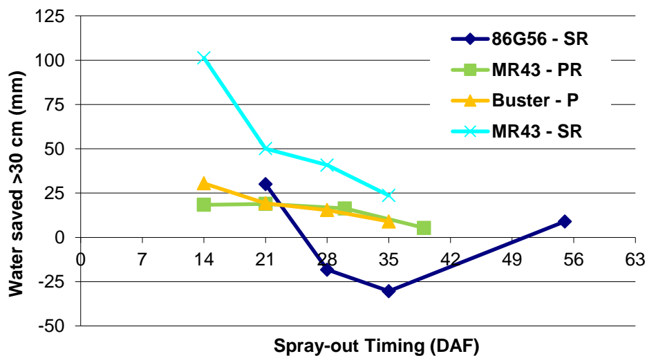
Soil moisture saved 'Southern' sites 2008
