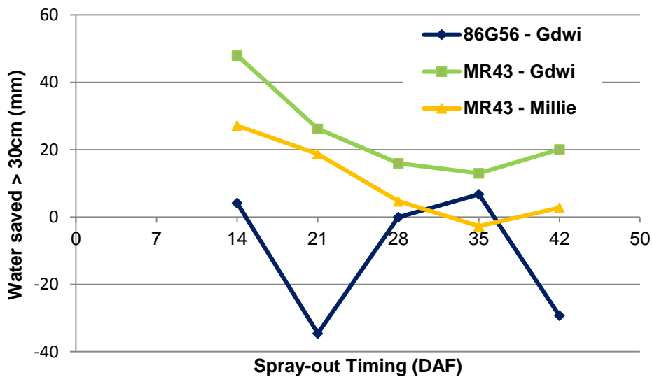
Soil moisture saved 'Southern' sites 2008
